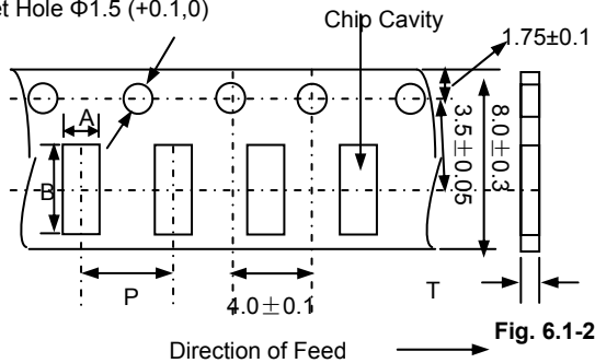
Paper Tape
